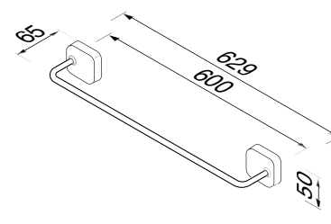
912407-02-60 Wandhanddoekhouder 60 cm Towel rail 60 cm Handtuchreck 60 cm Porte serviettes 60 cm Toallero 60 cm
