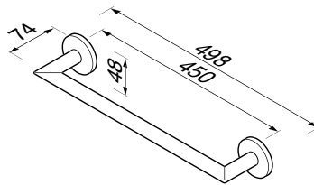
916507-02-45 Wandhanddoekhouder 45 cm Towel rail 45 cm Wandhandtuchhalter 45 cm Porte serviettes 45 cm Toallero 45 cm
