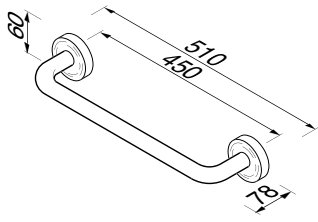
915531-45 Wandhaddoekhouder 45 cm Towel rail 45 cm Wandhandtuchhalter 45 cm Porte serviettes 45 cm Toallero 45 cm
