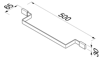
918407-02-50 Wandhanddoekhouder 50 cm Towel rail 50 cm Handtuchhalter 50 cm Porte serviettes 50 cm Toallero 50 cm
