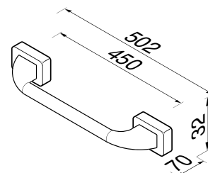
917031-45 Wandhanddoekhouder 45 cm Towel rail 45 cm Wandhandtuchhalter 45 cm Porte serviettes 45 cm Toallero 45 cm
