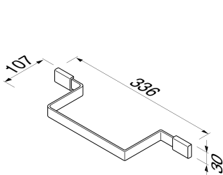
918404-02 Handdoekring Towel ring Handtuchring Anneau porte-serviettes Toallero anillo
