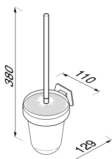
915117 Toiletborstelhouder, wandmodel Toilet brush holder, wall mounted Toilettenbürstengarnitur, zur Wandmontage Porte-balai, fixation murale Escobillero
