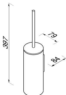
917311-04 Toiletborstelhouder, wandmodel Toilet brush holder, wall mounted Toilettenbürstengarnitur, zur Wandmontage Porte-balai, fixation murale Escobillero, montado a pared
