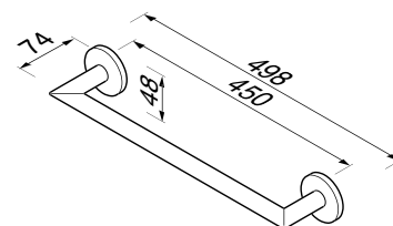
916507-05-45 Wandhanddoekhouder 45 cm Towel rail 45 cm Wandhandtuchhalter 45 cm Porte serviettes 45 cm Toallero 45 cm
