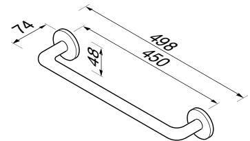
916576-02-45 Wandhanddoekhouder 45 cm Towel rail 45 cm Wandhandtuchhalter 45 cm Porte serviettes 45 cm Toallero 45 cm
