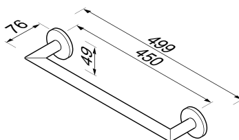
916507-06-45 Wandhanddoekhouder 45 cm Towel rail 45 cm Wandhandtuchhalter 45 cm Porte serviettes 45 cm Toallero 45 cm
